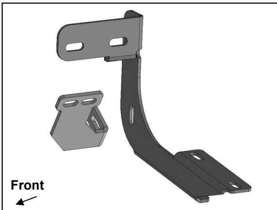
(Figure 6) Driver/left front/center Mounting Bracket and (1) driver/left front/center Support Bracket. NOTE: Driver/left front/center Support Brackets are the same as the passenger/right rear Support Bracket.
