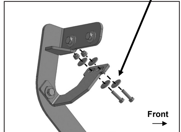
(Figure 14) Models with factory holes in pinch weld only. Attach Support Bracket to back of pinch weld.
