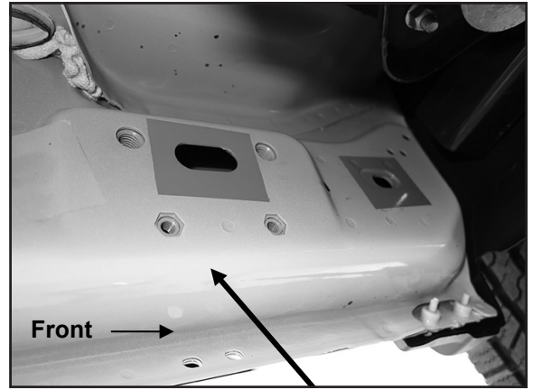
(Figure 10) Example of model with factory installed threaded mounting holes.
