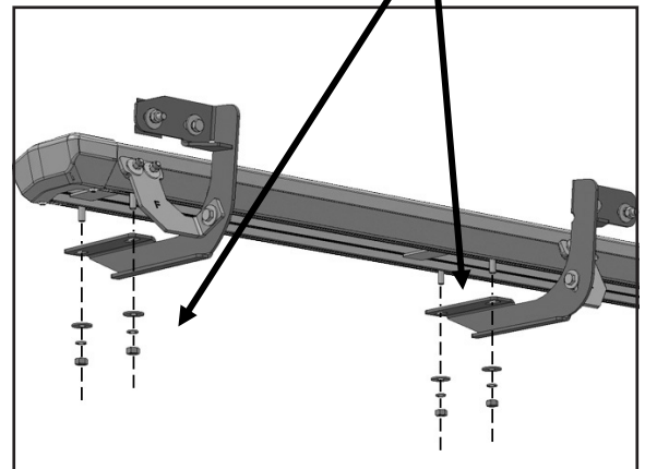
(Figure 23) Attach the driver/left Running Board to the center and rear Brackets.
