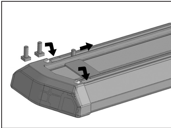
(Figure 21) Insert (3) 8mm T-Bolts into each channel in the bottom of the Running Board.
