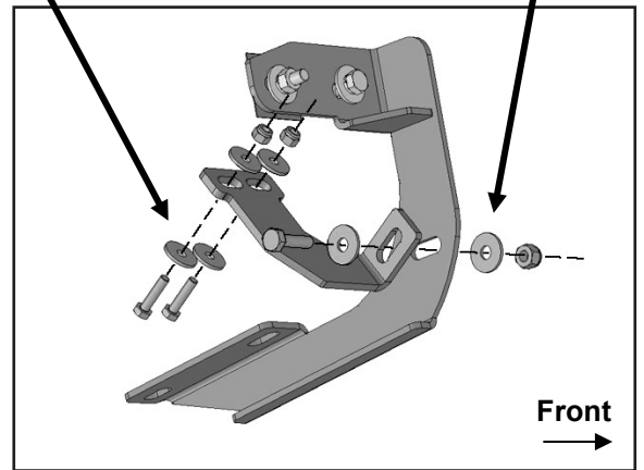
(Figure 19) Attach (1) driver/left rear Support Bracket to rear facing side of driver/left rear Mounting Bracket.
