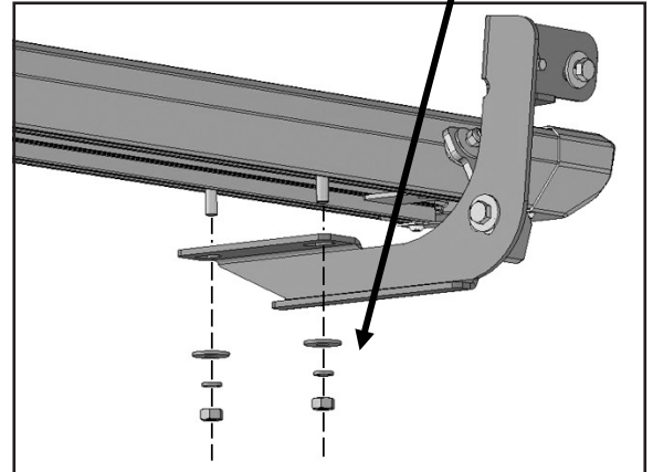
(Figure 22) Attach the Running Board to the driver/left front Mounting Bracket.
