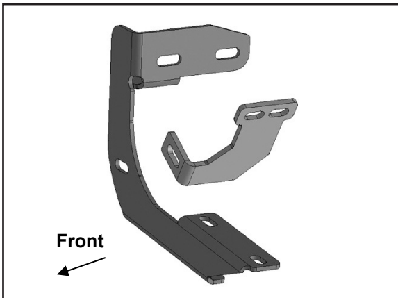
(Figure 17) Driver/left rear Mounting Bracket and Support Bracket.
