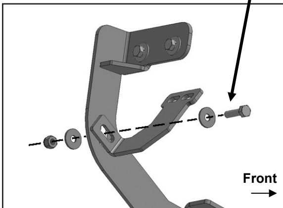
(Figure 13) Attach (1) Driver/left front Support Bracket to front facing side of Front Bracket.
