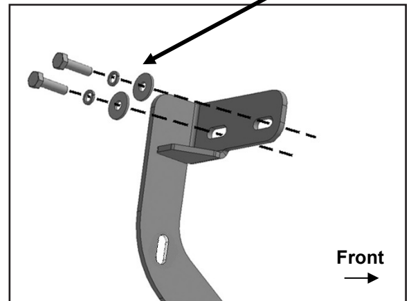
(Figure 11) Models with factory installed threaded holes in mounting locations. Attach driver/left front Mounting Bracket directly to threaded holes.
